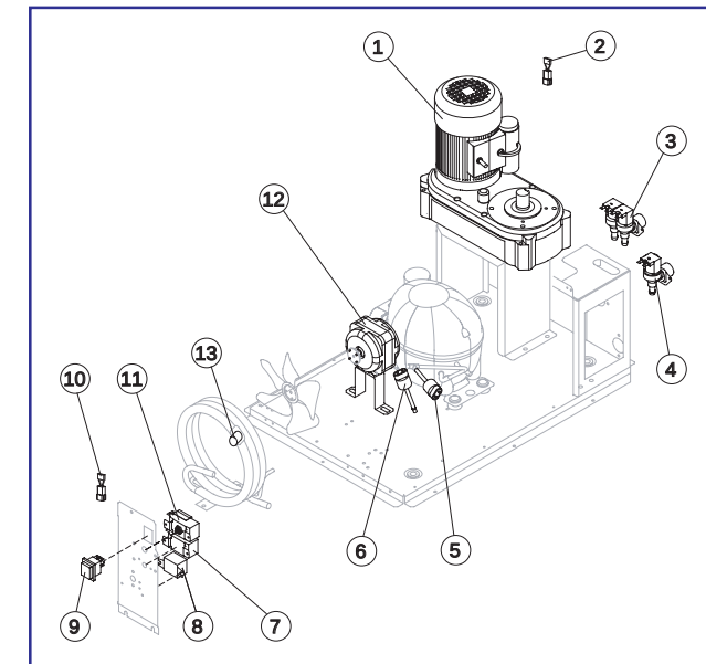
ELECTRIC PARTS
