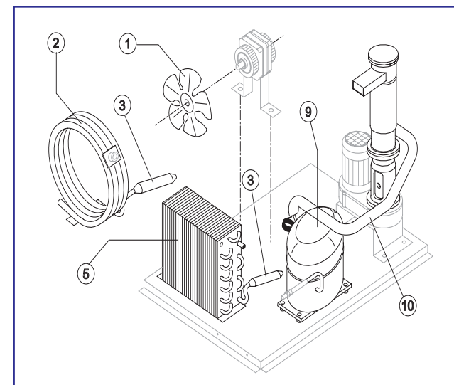
COOLING SYSTEM
