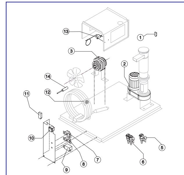
ELECTRIC PARTS
