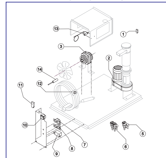
ELECTRIC PARTS
