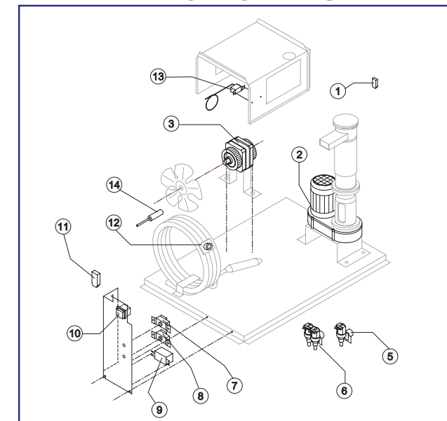
ELECTRIC PARTS
