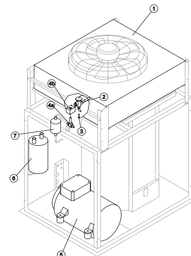
ELECTRIC PARTS
