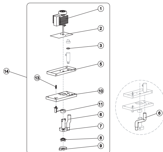
PUMP
