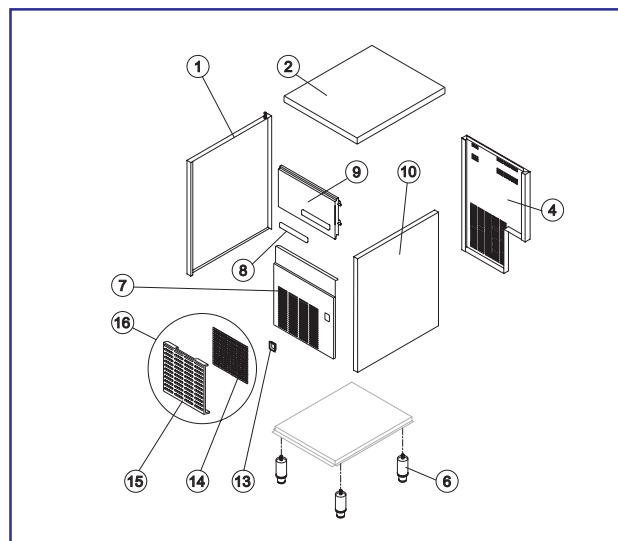
INVOLUCRO
